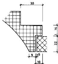
DETAIL ANTRITT
