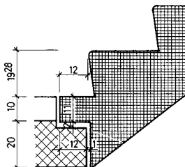
DETAIL ANTRITT
