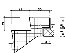
DETAIL AUSTRITT
