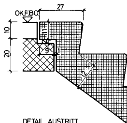
DETAIL AUSTRITT
