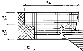
DETAIL AUSTRITT
