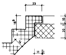
DETAIL AUSTRITT
