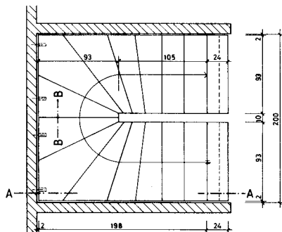
DETAIL ANTRITT
