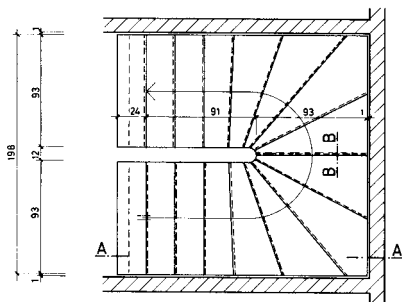
DETAIL ANTRITT
