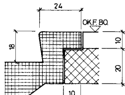
DETAIL AUSTRITT
